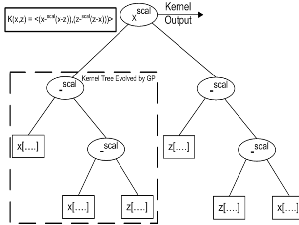
Figure 2. Example of a Kernel found on the Wisconsin Breast Cancer Dataset
