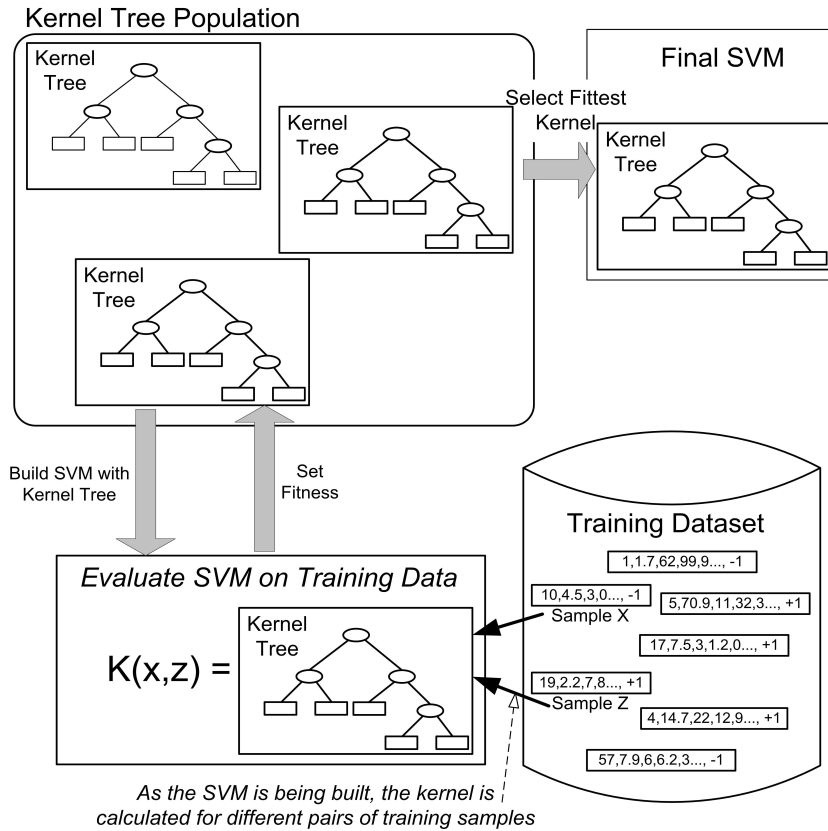
Figure 1. The Genetic Kernel SVM
